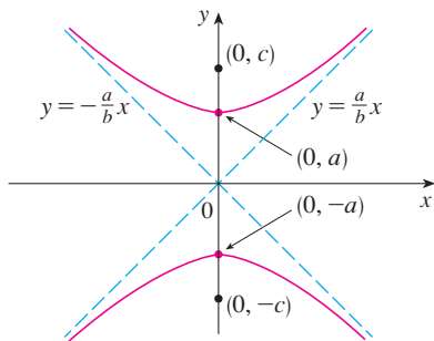
FIGURE 13 \frac{y^2}{b^2} - \frac{x^2}{a^2} = 1
